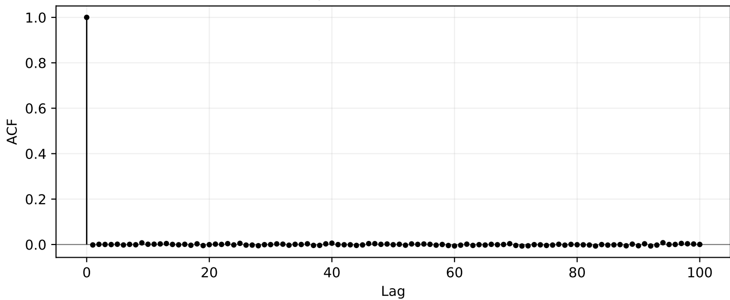
\beta_0 running mean
